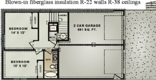
BASEMENT PLAN SCALE : NTS 592 SQ. FT.
