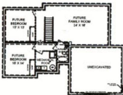
BASEMENT PLAN SCALE: 1/8" = 1'-0"
