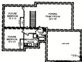
BASMENT PLAN SCALE 1/8" = 1'-0"
