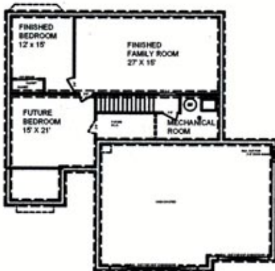
BASEMENT PLAN SCALE: 1/8" = 1'-0" 1188 SQ. FT.
