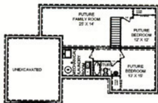
BASEMENT PLAN SCALE: 1/8" = 1'-0"
