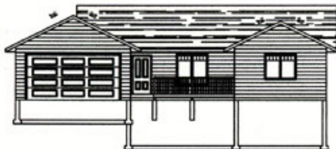
FRONT ELEVATION SCALE: NTS
